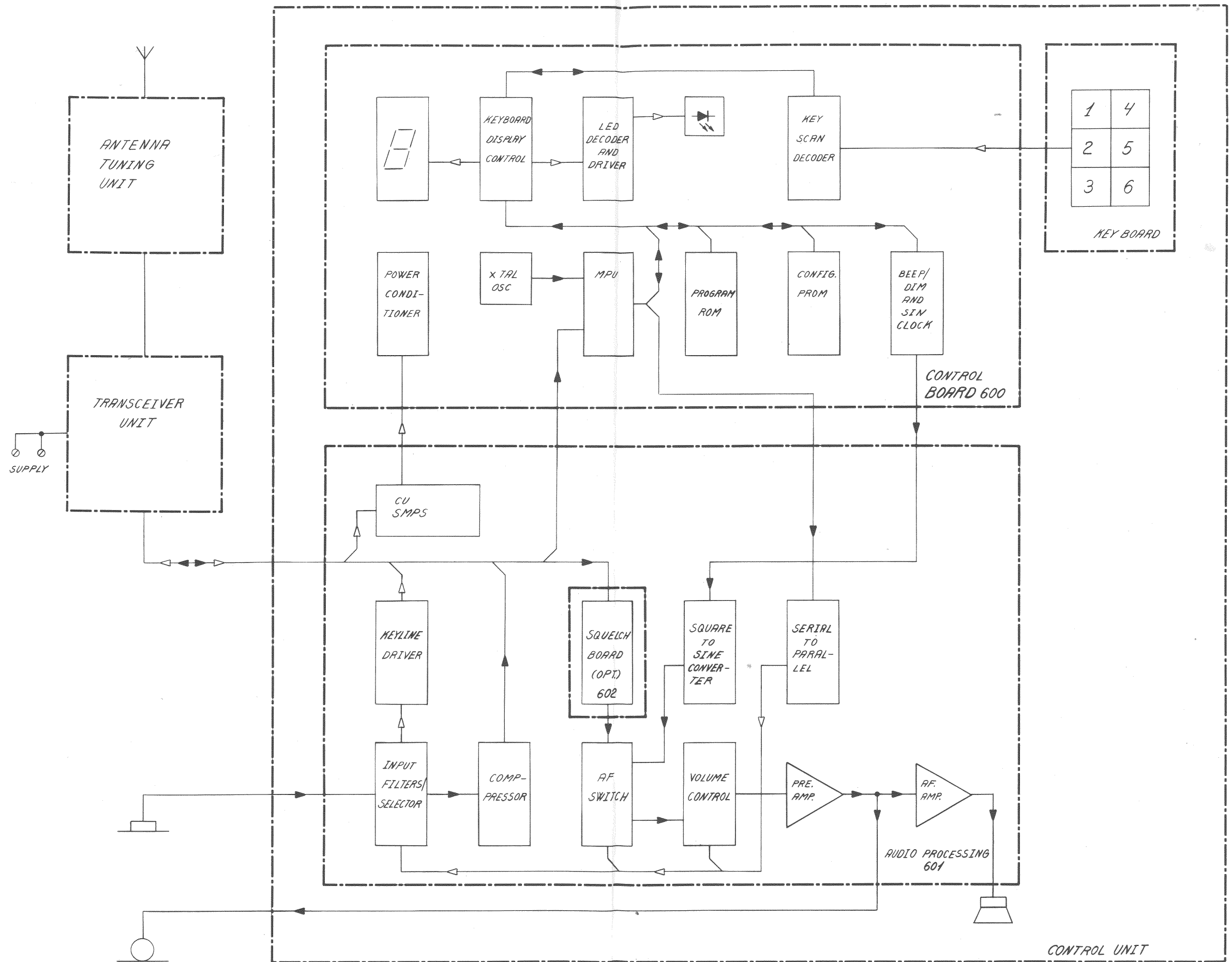
TRP 8250S BLOCK DIAGRAM, CONTROL UNIT VERSION 1A
